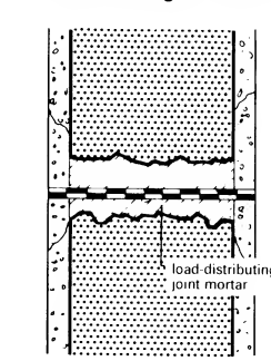
⑫ Retrofitted horizontal (damp-proof course)
